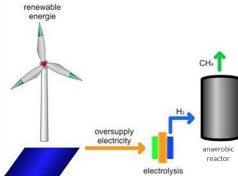
Figure 5: Use of surplus electricity to biogas plants via hydrogen
